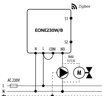
b) Connection diagram to pump / actuator
