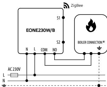
a) Connection diagram for gas boiler
