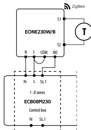
c) Connection diagrams to the control box
