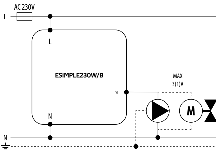
a) Connection diagram to pump / actuator
