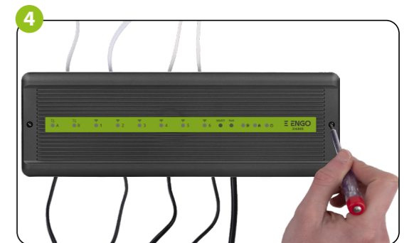
After making sure all wires are properly connected, mount the top cover and plug the wiring centre to the 230 V power supply - the red "Power" diode will light up.
