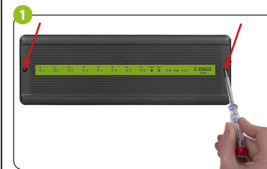
Remove the top cover of the control box
